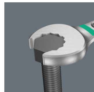
The double hexagon geometry on the open end and ring sides secures the positive connection with the screw head or bolt and reduces the risk of slipping.
