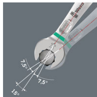
Thanks to the open end side offset by 7.5°, double hexagon geometry and an adjusted application method (placement - screwdriving - turning - replacement - screwdriving - turning, etc), even screwdriving challenges allowing a return angle of less than 30° can be solved.
