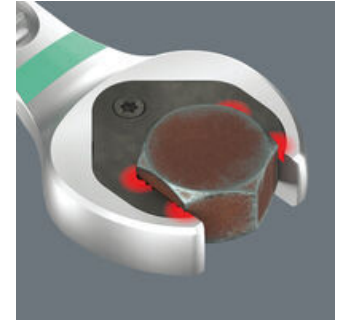
Double-hex geometry
